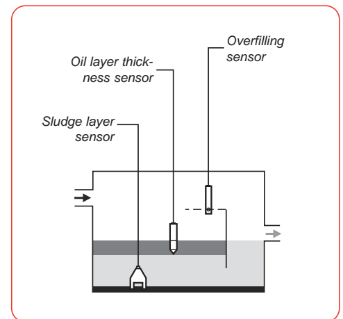
Oil-water separator
