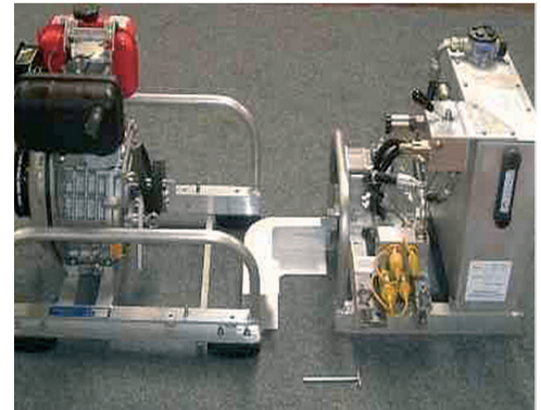
Power pack showing two part configuration for easy handling
