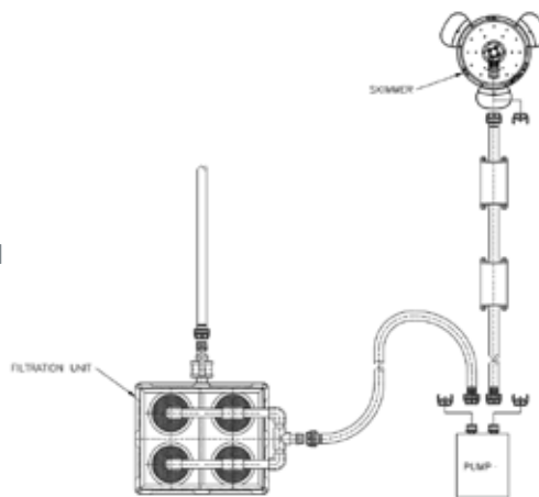
Above: Skimmer system layout
