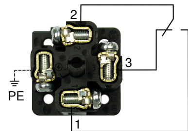
Connection: Contact position in the under-run state
